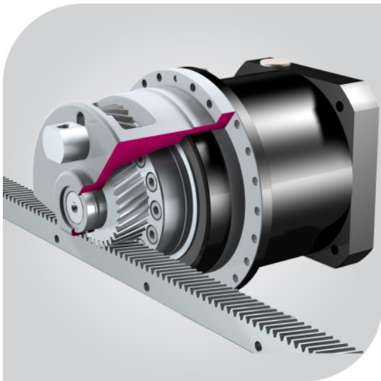
ZTRS-PH Gear Rack Drive
